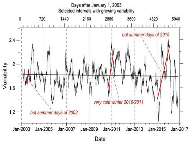
Figure 2 – Variability of SAT data at the Sporilov station (running average for 100 consecutive days. Intervals with large variability are highlighted (taken from Čermák et al., 2019)
